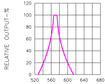
Fig.2 SPECTRAL RESPONSE
